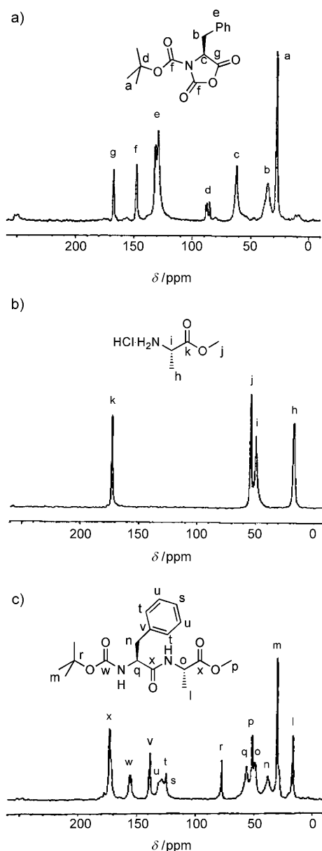
Figure 1. CP/MAS solid-state ^{13}\text{C} NMR analysis of a) Boc-Phe-NCA ( 1c ), b) HCl·H 2 N-Ala-OMe ( 2c ), and c) crude Boc-Phe-Ala-OMe.
